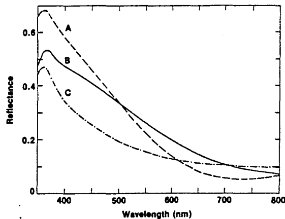
Fig. 3. Spectral variation of the reflectance of a 140-nm thick layer of SiO 2 on Si: A, TE polarized 45° angle of incidence; B, 0° incidence; C, TM polarized 45° incidence.
