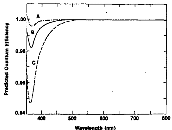
Fig. 4. Predicted quantum efficiency of the four photodiode light-trapping devices used in this study: A, TM polarized input; B, unpolarized; C, TE polarized.
