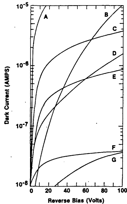
Fig. 8. Dark current vs reverse bias voltage for several different types of silicon photodiode: A,F,G, UV-enhanced boron doped p-n type; B,D, inversion layer (undoped) type; C,E, phosphorus doped n-p type. All are without guard rings.
