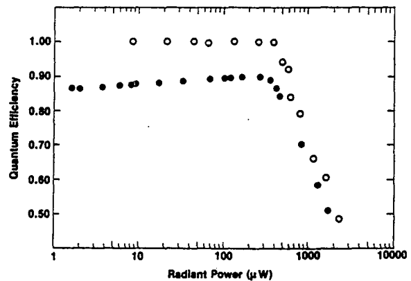
Fig. 6. Measured quantum efficiency as a function of radiant power level at 406.7 nm \circ and 799.3 nm \bullet .
